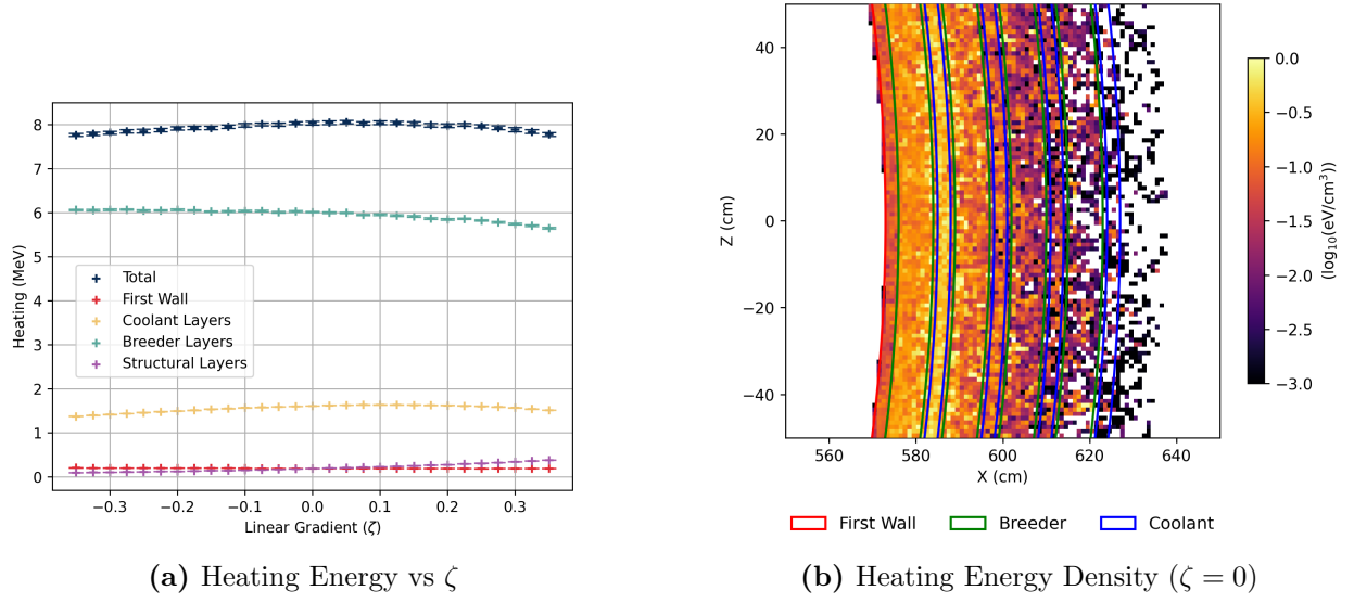
Figure B2: Total nuclear heating deposition rates and a corresponding spatial concentration within the discrete blanket layers.
